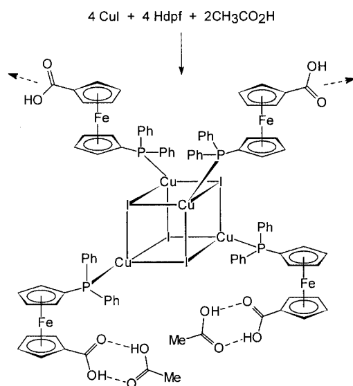
Scheme 8. Preparation and structure of the solvated heterocubane 28 ·2CH 3 CO 2 H. Dashed arrows indicate where propagation of the infinite, hydrogen-bonded chains occurs.
