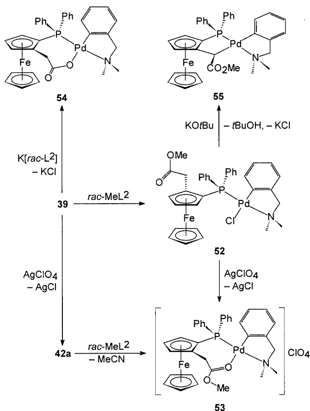
Scheme 16. Synthesis of \{[(\text{dimethylamino})\text{methyl}]\text{phenyl-}\kappa^2\text{C}^1,\text{N}\} palladium(II) complexes with “L 2 family” ligands.
