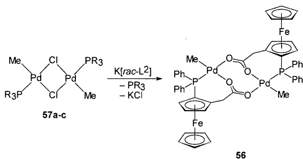
Scheme 17. Formation of dipalladium(II) complex 56 featuring a bridging tridentate [\text{rac-L}^2]^- anion [ \text{PR}_3 = \text{PMe}_3 (a), \text{PPh}_3 (b), and \text{PFur}_3 , where Fur = fur-2-yl (c)].
