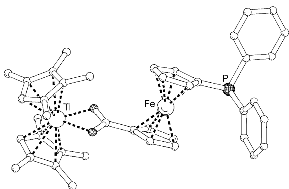
Figure 6. Molecular structure of bis(metalloocene) complex 38 .
