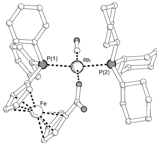
Figure 5. View of the molecular structure of 36a . Hydrogen atoms are omitted.
