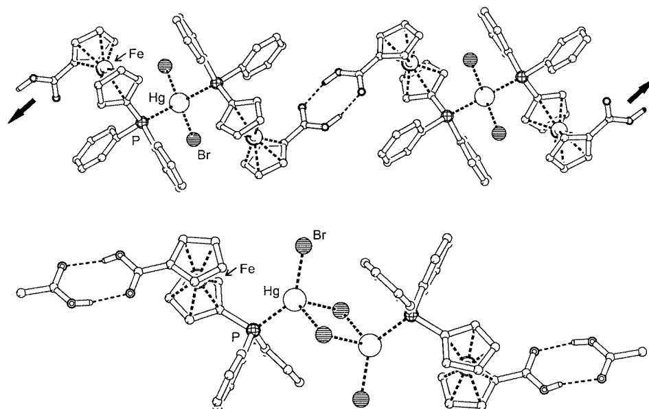
Figure 3. Views of the molecular structures of 26b (top) and 27b ·4CH 3 CO 2 H (bottom). The O···O hydrogen bonds are shown as dashed lines and the propagation of the chains in the structure of 26b is indicated with arrows. The dimers (CH 3 CO 2 H) 2 present in the structure of the solvate are not shown for clarity.
