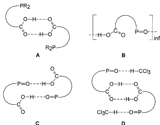
Scheme 21. Hydrogen bonding patterns observed for phosphorus-substituted ferrocenecarboxylic acids.
