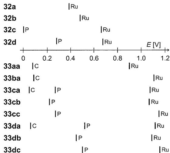
Figure 4. Chart diagram of the anodic redox potentials observed for 32 and 33 in dichloromethane solutions. The redox potentials were determined as an average of the anodic and cathodic peak potentials and given relative to the ferrocene/ferricenium reference. The values are distinguished as follows: the symbol Ru indicates a ruthenium-centered oxidation, while C and P denote the ferrocene/ferricenium potentials for carbene and phosphanyl-ferrocenyl groups, respectively. For compound labels see Scheme 9.
