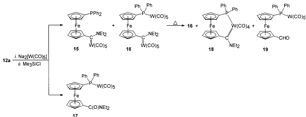
Scheme 7. Carbene-forming reactions with 12a and pentacarbonyltungstate.
