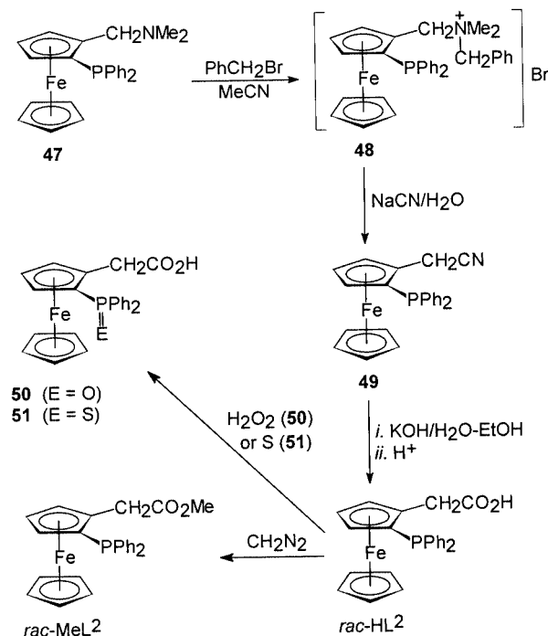
Scheme 15. Preparation of rac -HL 2 and its derivatives.
