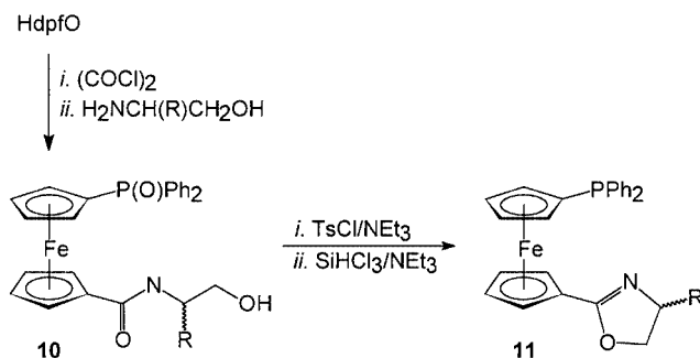
Scheme 5. Synthesis of ferrocenyl-oxazolines [ R = (S) - i Pr, ( R )- i Pr, ( S )- t Bu, ( R )-Ph].
