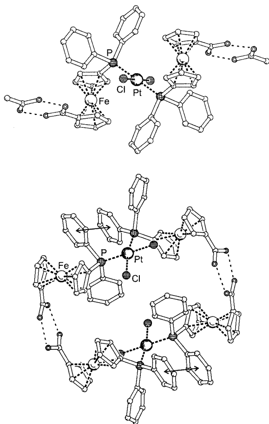
Figure 2. Views of the repeating units in the crystals of 22 ·2CH 3 CO 2 H (top) and 23 ·(2+ x )CH 2 Cl 2 (bottom). The O···O hydrogen bonds are shown as thin dashed lines and the \pi\cdots\pi stacking interactions of the phenyl rings are indicated by double arrows. Hydrogen atoms and solvating dichloromethane (for the latter compound) are omitted for clarity.
