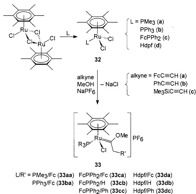
Scheme 9. Synthetic route to cationic (methoxycarbene)ruthenium compounds 33 .
