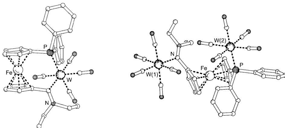
Figure 1. Views of the molecular structures of complexes 18 (left) and 16 (right).
