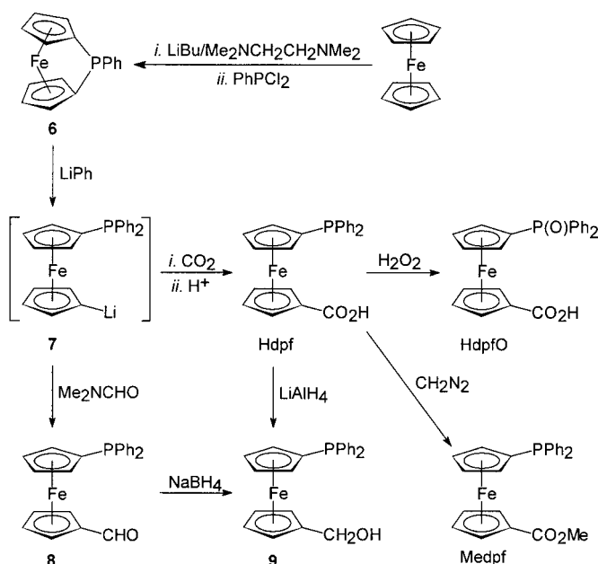
Scheme 3. Synthesis of Hdpf and related compounds.
