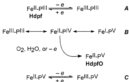
Scheme 4. Schematic depiction of the ECE electrochemical behaviour observed for Hdpf.
