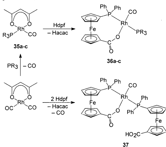
Scheme 10. Preparation of rhodium(I) complexes with O,P -chelating phosphanyl-carboxylate \text{dpf}^- [ \text{PR}_3 = \text{PCy}_3 ( a ), \text{PPh}_3 ( b ), and \text{FcPPh}_2 ( c ); Cy = cyclohexyl].
