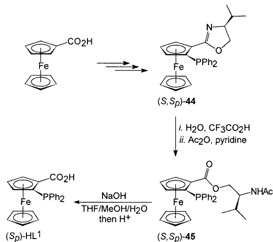
Scheme 13.
