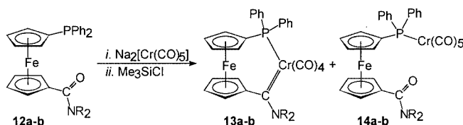
Scheme 6. Preparation of (carbene)chromium(0) compounds [ \text{NR}_2 = \text{NEt}_2 ( a ) and morpholin-4-yl ( b )].
