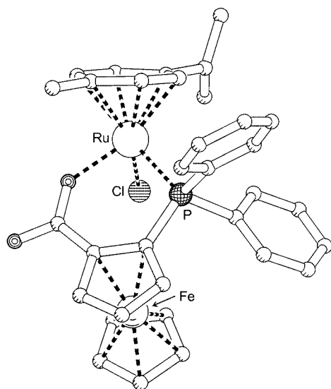
Figure 7. View of the molecular structure of (R_{Ru},S_p)\text{-46} as obtained for the solvate (R_{Ru},S_p)\text{-46}\cdot 0.7\text{CH}_2\text{Cl}_2 . Molecules of solvating dichloromethane are not shown.
